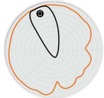
Figure 5. H550 5GHz Elevation Antenna Patterns
